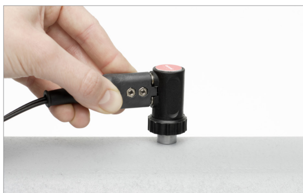
Wall thickness gauge NT in use (alternative design)
