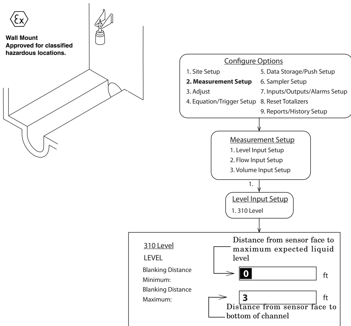
Figure 2-14 Configuring ultrasonic level measurement
